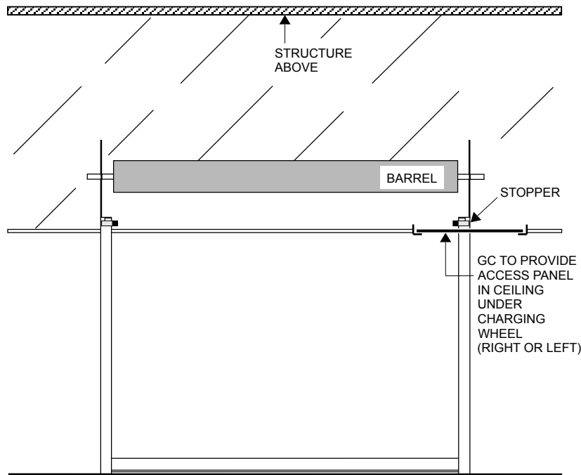
ELEVATION COIL SIDE ( INTERIOR )
