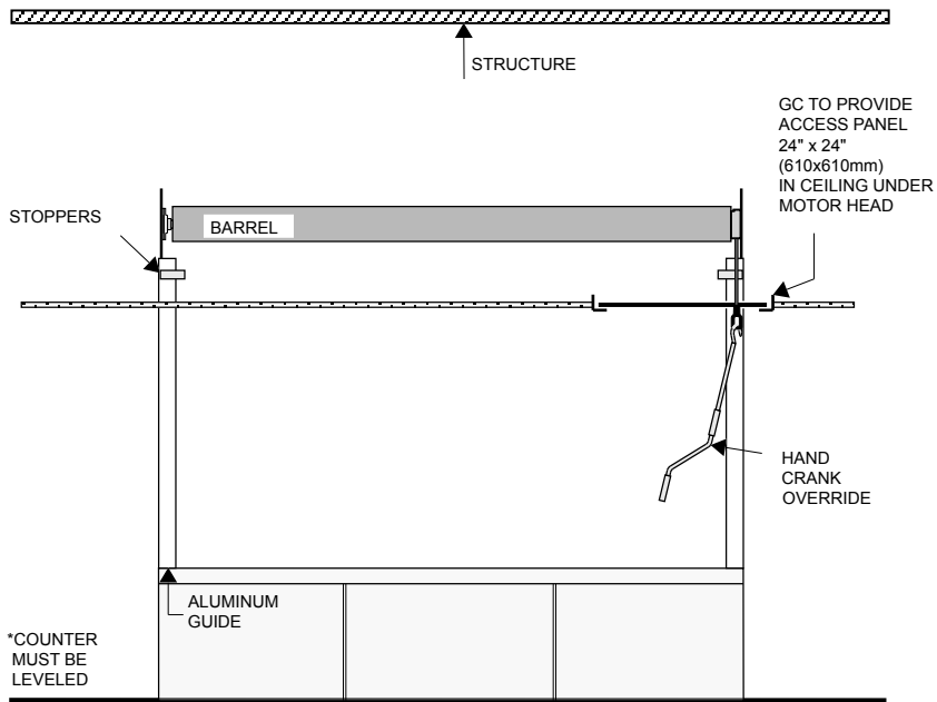
( INTERIOR ) ELEVATION COIL SIDE
