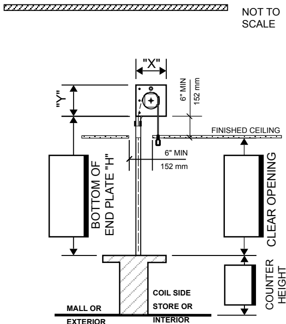
SECTION ( COUNTER )
