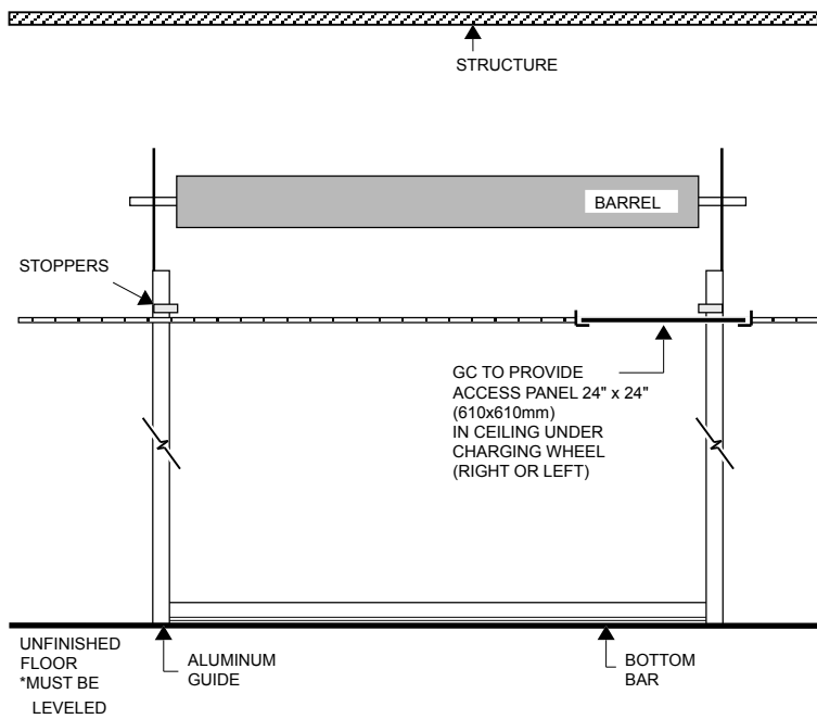
ELEVATION COIL SIDE ( INTERIOR )
