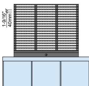
SLIM ROLL-AIR (Perforated)
